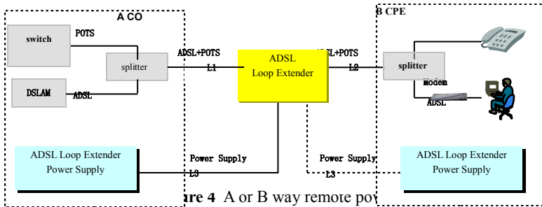
Figure 4 A or B way remote power supply
