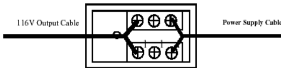
Figure5 WH-AE-AECB1P Connector Wiring Diagram
